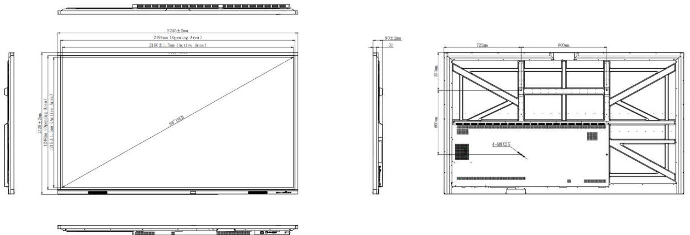
98": ST-98-CONNECT-PRO5
